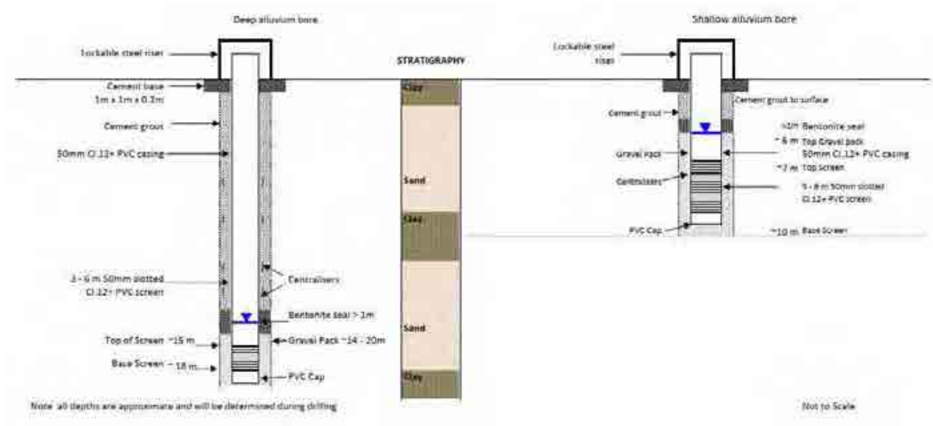
Figure 22 Indicative bore construction design for GDE&W specific monitoring bores
